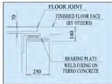
CONCRETE SUPPORT BEAM
