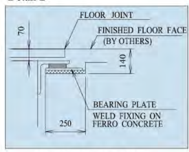
CONCRETE SUPPORT BEAM
