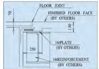
IRON FRAME SUPPORT BEAM
