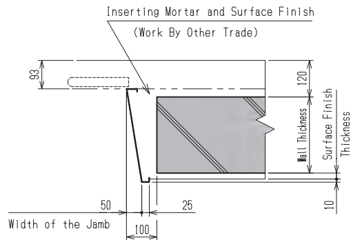
Optional (Right Side of the Wide Jamb)
