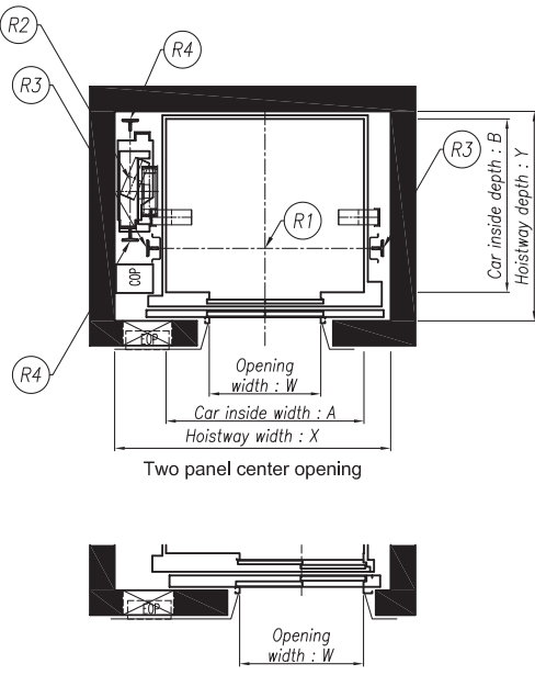
Hoistway Plan 800kg <= Capacity <= 2000kg
