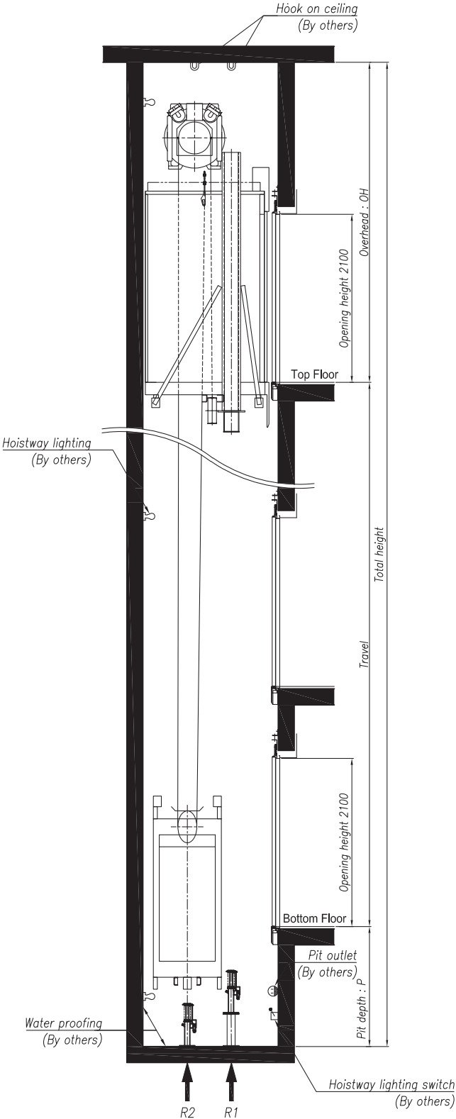
Hoistway Sectional Elevation
